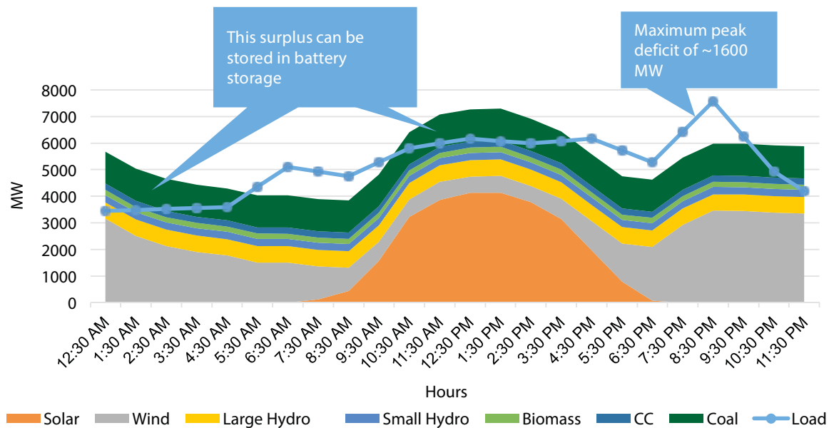
Figure 19: 2040 - Typical daily demand-supply scenario
