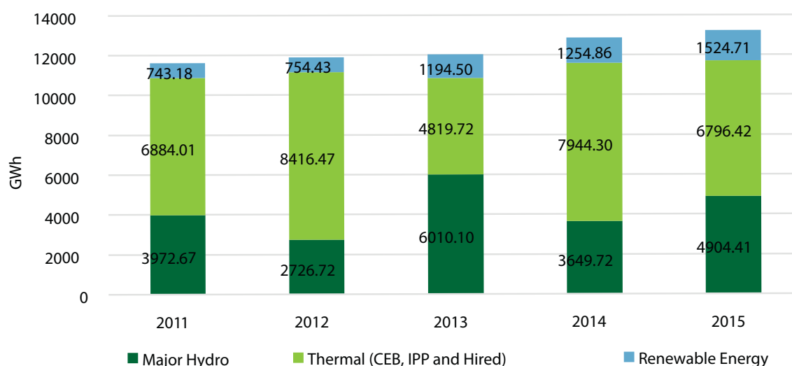
Figure 8: Sri Lanka Electricity Generation Mix Trend (2011-15)
