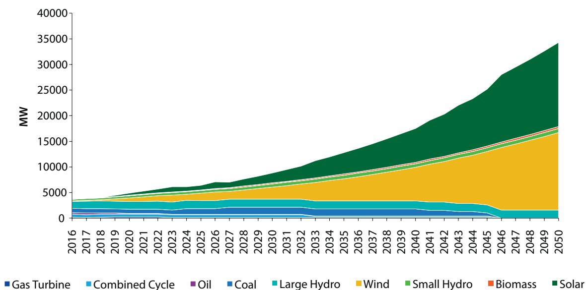
Figure 11: Sri Lanka 2050 electricity generation mix: 100 percent RE
