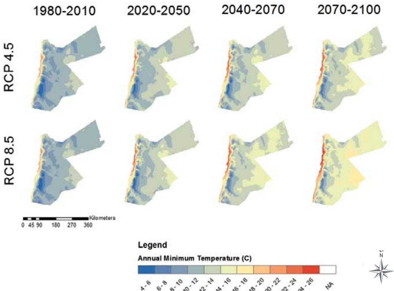
Figure 4.9: Projected average minimum temperature (°C) over Jordan using the reference model, for 2035, 2055 and 2085 times-horizons and for RCP 4.5 and 8.5
