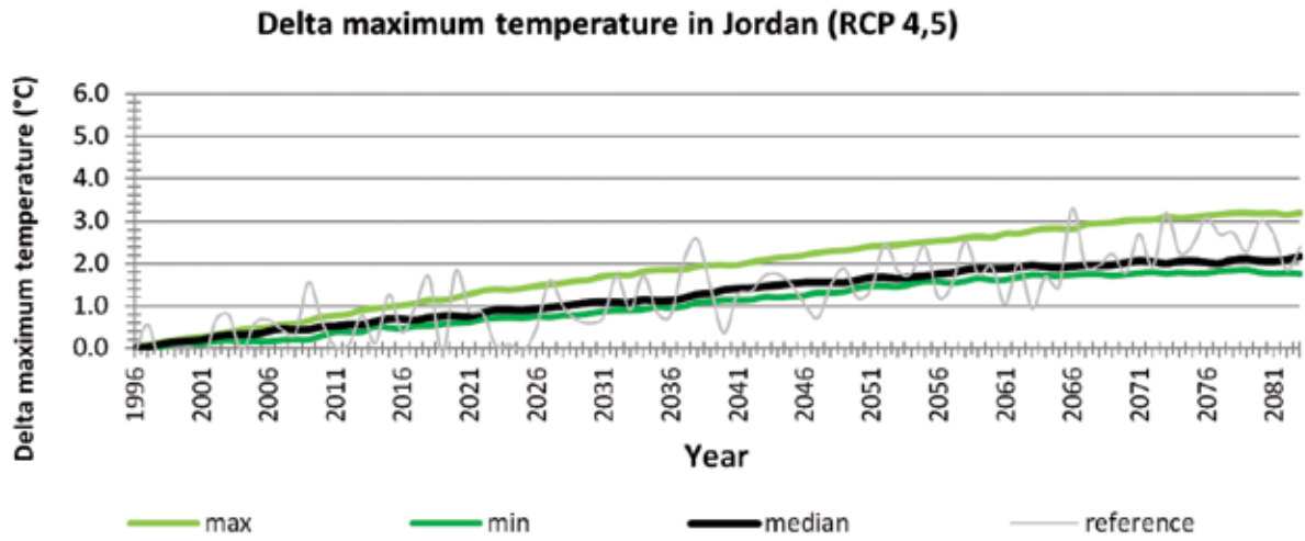
Figure 4.12: Projected changes in maximum temperature (°C) over Jordan for RCP 4.5 and 8.5
