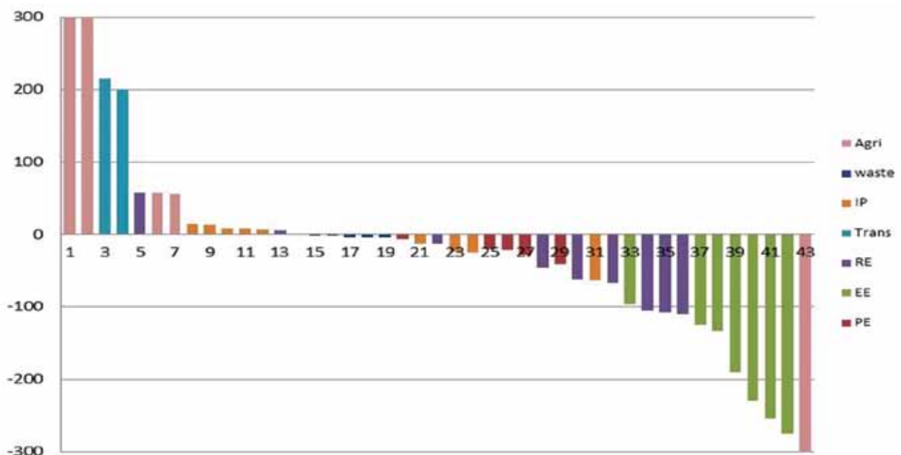
Figure 3.10: Abatement marginal cost for all mitigation measures ranked from the highest reduction cost to the lowest (for projects 1, 2 and 43 reduction costs are: 1922, 1356 and -1335 respectively)
