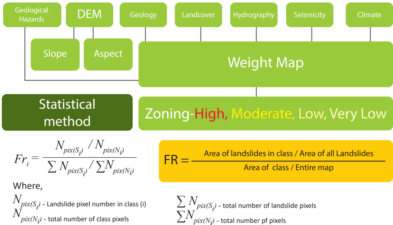
Figure 11. Statistical method for landslide hazard mapping
