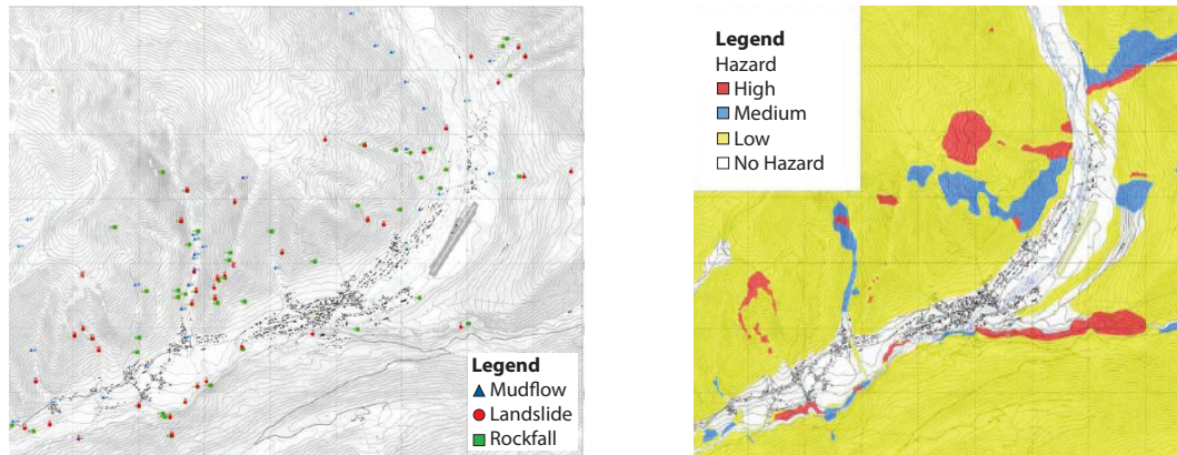
Figure 19. Map of the geological hazard sources of the Mestia-Lendgeri area
