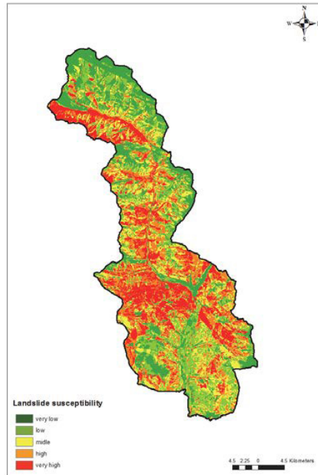
Figure 26. Geological Hazard (landslide, debris/mudflow, rockfall etc) susceptibility map
