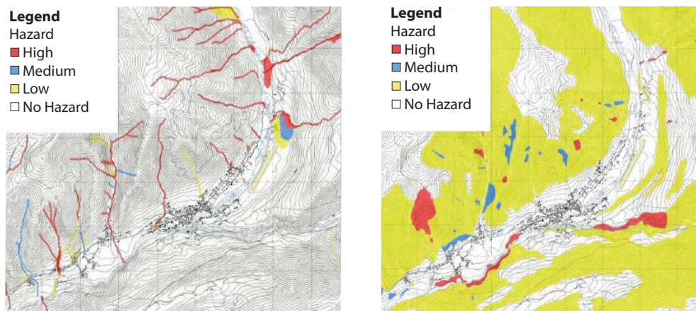
Figure 21. Mudflow hazard zoning map for the Mestia-Lendgeri area
