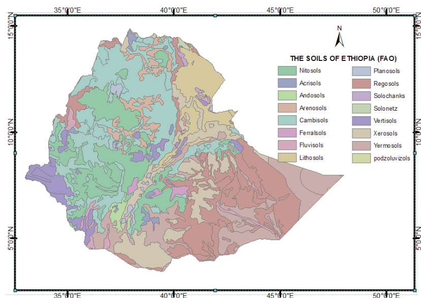
Figure: 1-4: The Soils of Ethiopia
