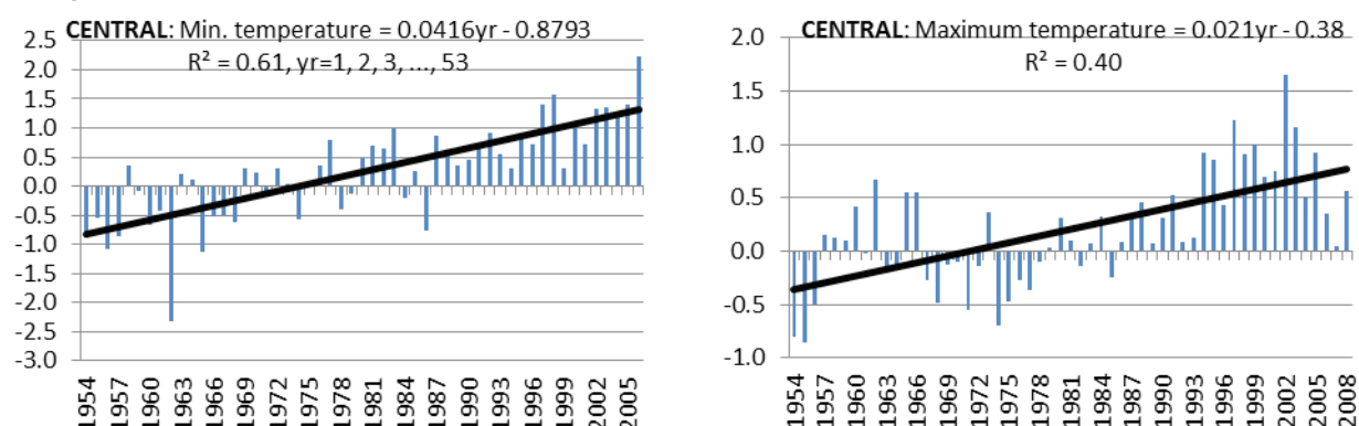
Figure ES 1-7: Inter-Annual Variation of the Mean Minimum and Maximum Temperatures for Central Ethiopia
