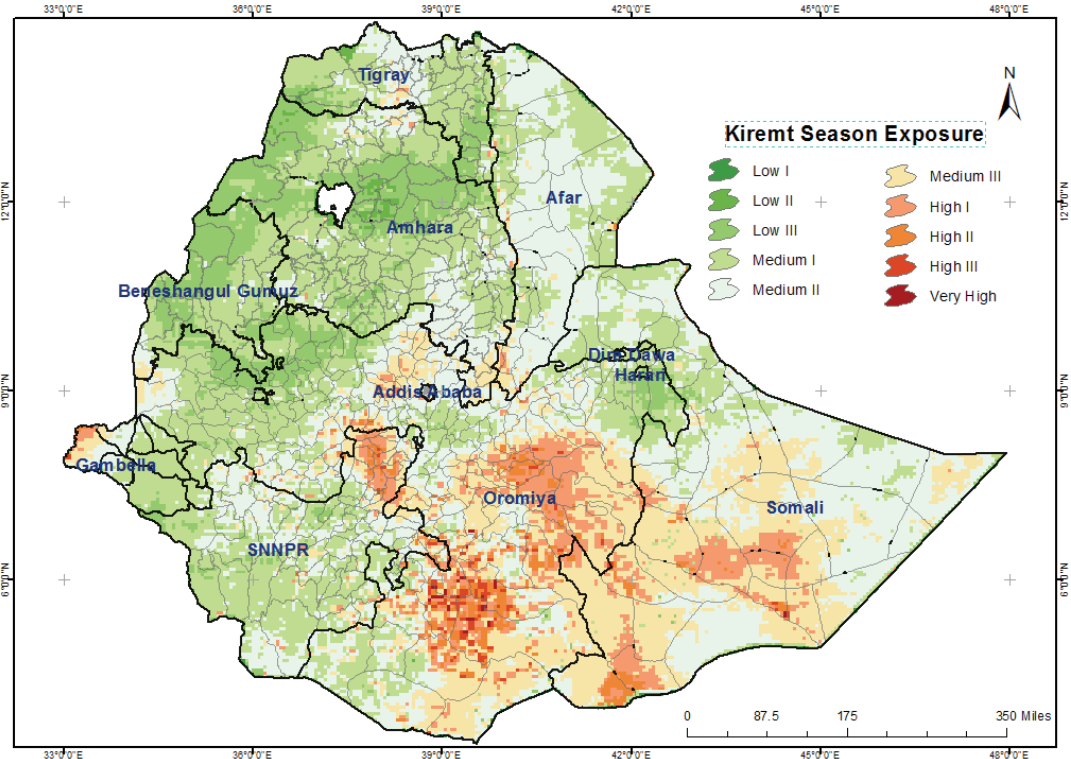
Figure 5-24: Kiremt Season Exposure
