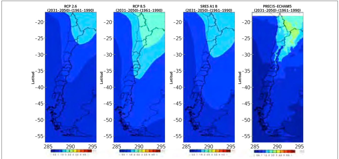
Figure 5. Maps of temperature change for RCP and SRES A1B (GCM and RCM) scenarios for the term 2031-2050 as compared to the term 1961-1990.
