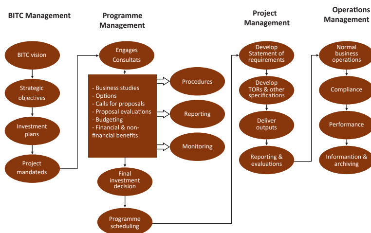
Figure 9: BEDP Workflow
