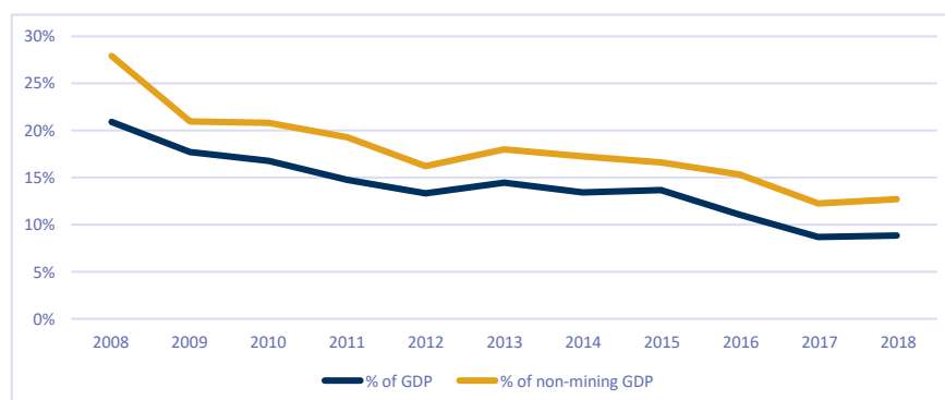
Figure 3: Exports of non-diamond exports of goods & services
