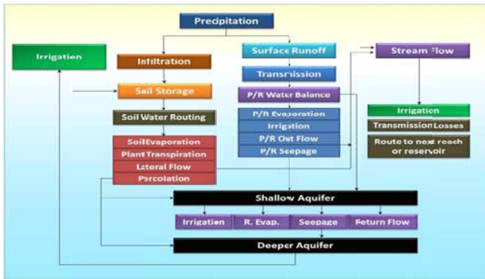
Figure (12): Schematic of pathways available for water movement in SWAT (Modified after Neitsch et. al.,2005)
