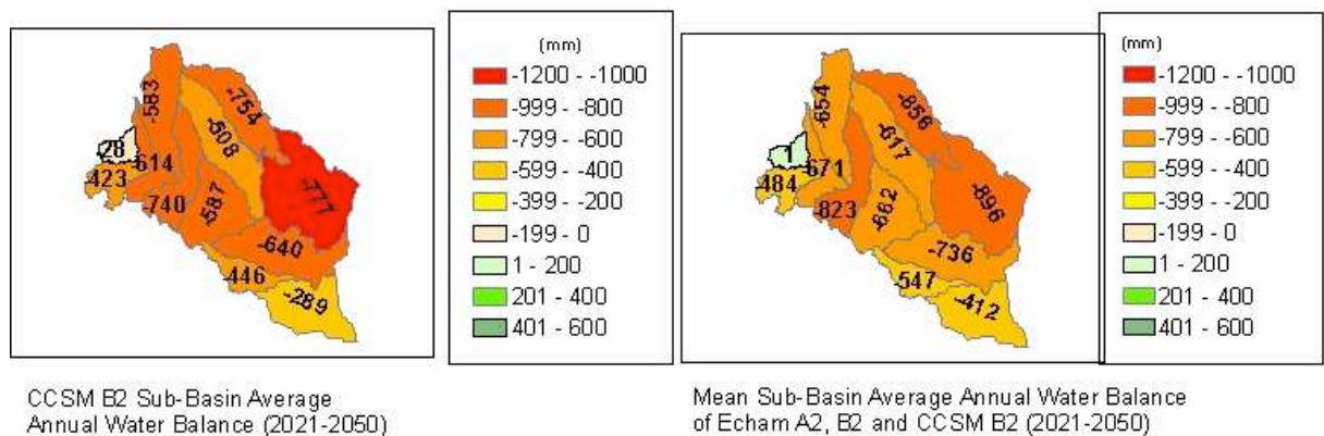
Figure 4.4 Observed average annual sub-basin water balance (mm rainfall - mm potential evaporation), based on data from rainfall gauges and class A-pans (1960-1980) and sub-basin average annual water balance as predicted for 2021-2050 by RCA3, driven by ECHAM4-A2, ECHAM4-B2, and CCSM3-B2, using the “Delta Change” approach. A negative water balance indicates that the annual rainfall is smaller than the annual atmospheric demand of moisture.
