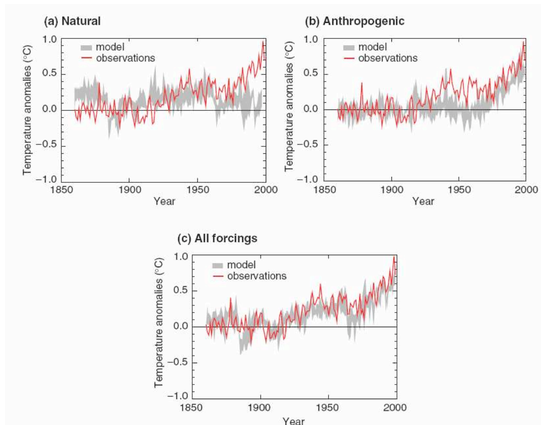
Figure 2.1. Measured (red) and simulated (grey) global mean surface temperature anomalies. The simulated data encompass an ensemble of four global climate model runs forced with natural (a) or anthropogenic (b) forcing as well a combination of both (c). The natural factors considered are solar and volcanic forcing. The anthropogenic factors include greenhouse gases, ozone changes and sulphate aerosols. [With permission from the Intergovernmental Panel of Climate Change, IPCC 2001. SPM, WGI, Figure 15.]
