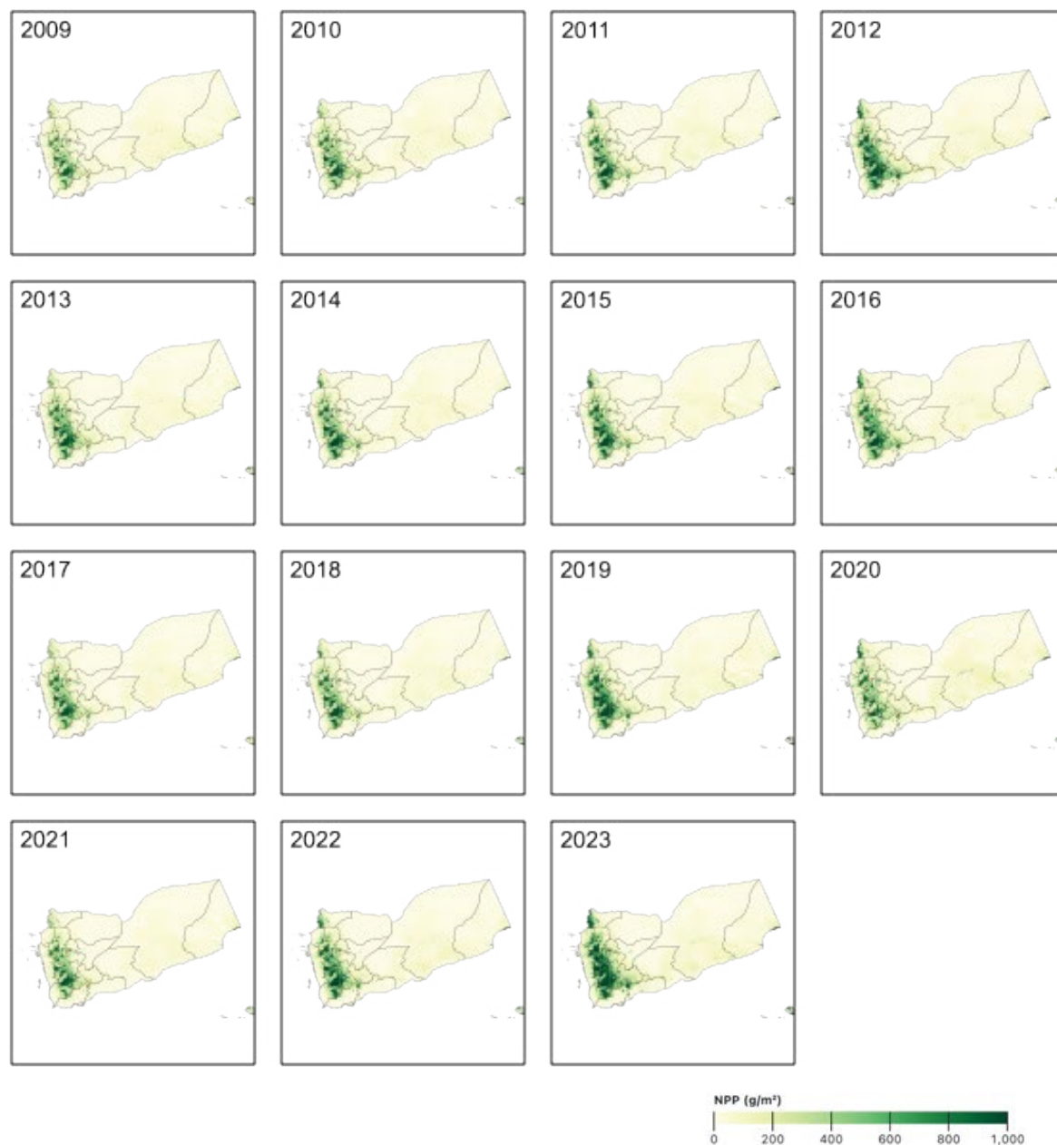
Figure A.1.1: Evolution of net primary productivity, 2009–2023
