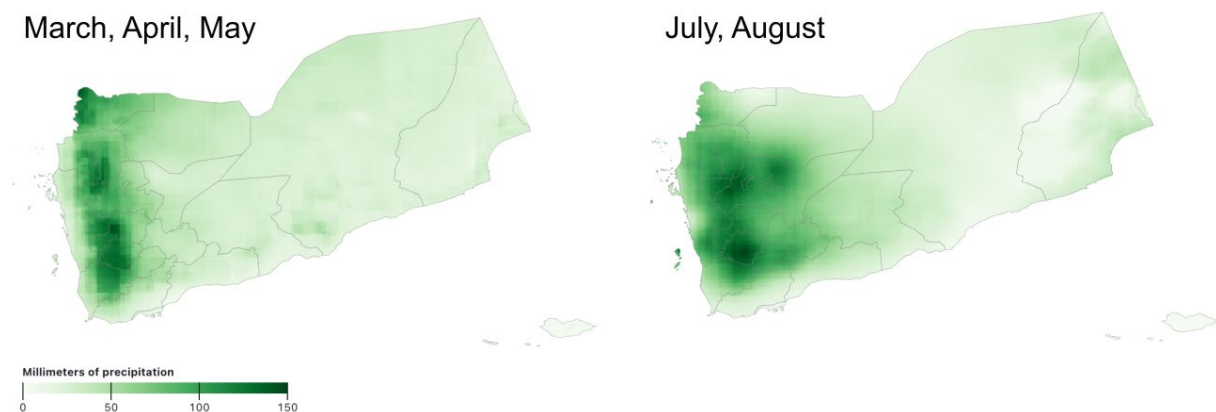
Figure 3: Seasonal annual average precipitation, 1981–2023
