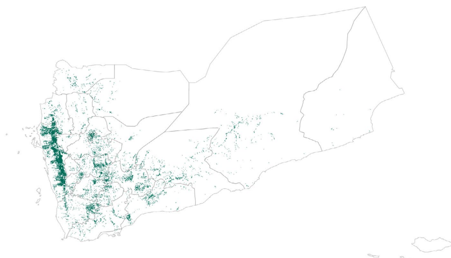
Figure 7: WorldCereal high-confidence crop areas in western Yemen, 2021
