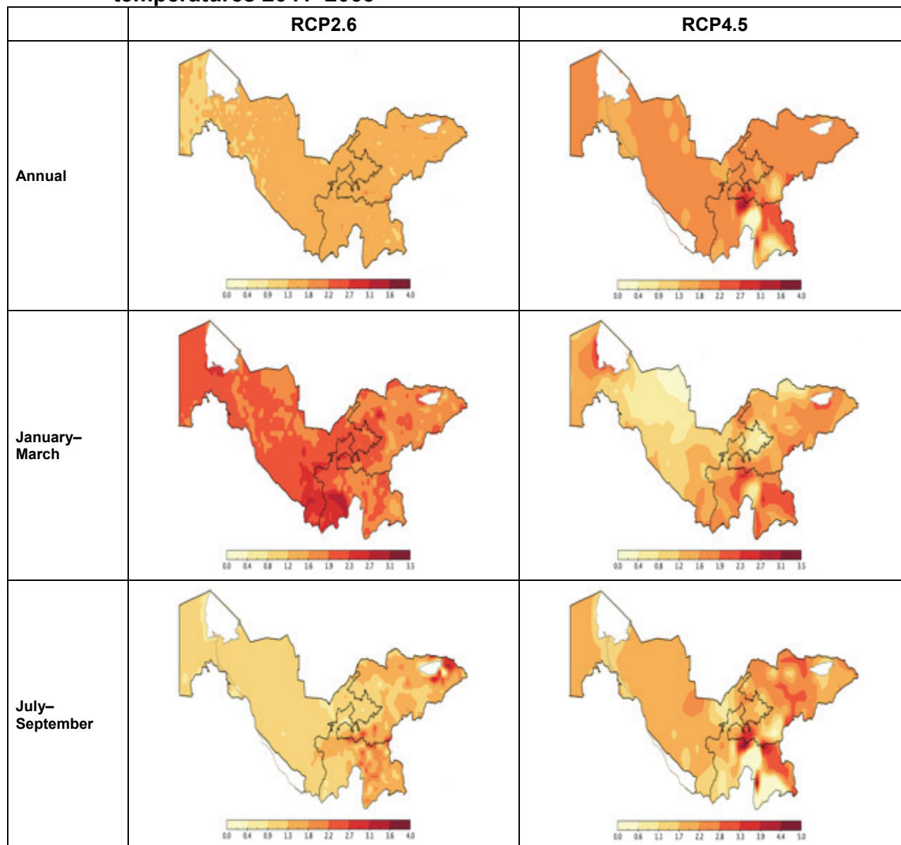
Figure 5 Projected mean anomalies in annual and seasonal maximum temperatures 2041–2065
