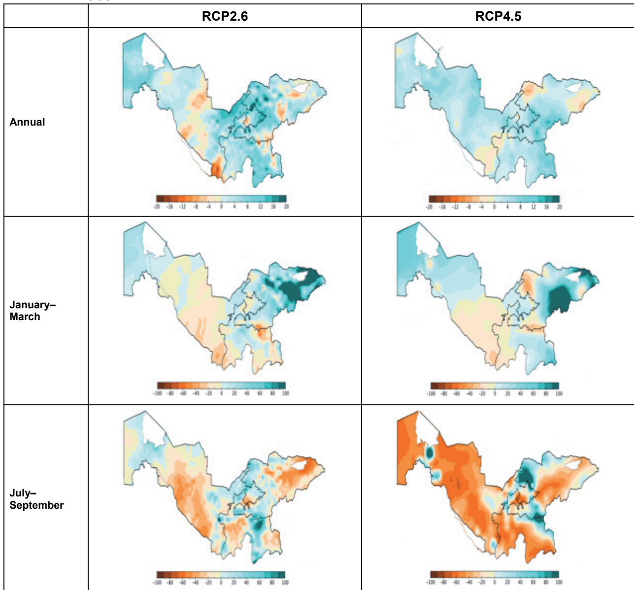
Figure 4 Projected percentage change in annual and seasonal precipitation 2036–2065
