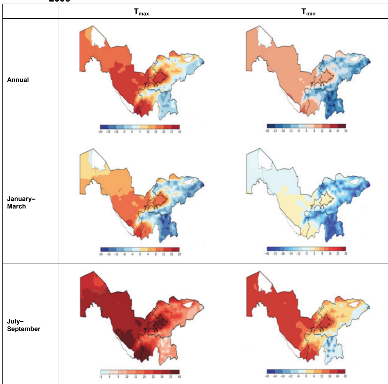
Figure 3 Annual and seasonal mean maximum and minimum temperatures 1981–2005
