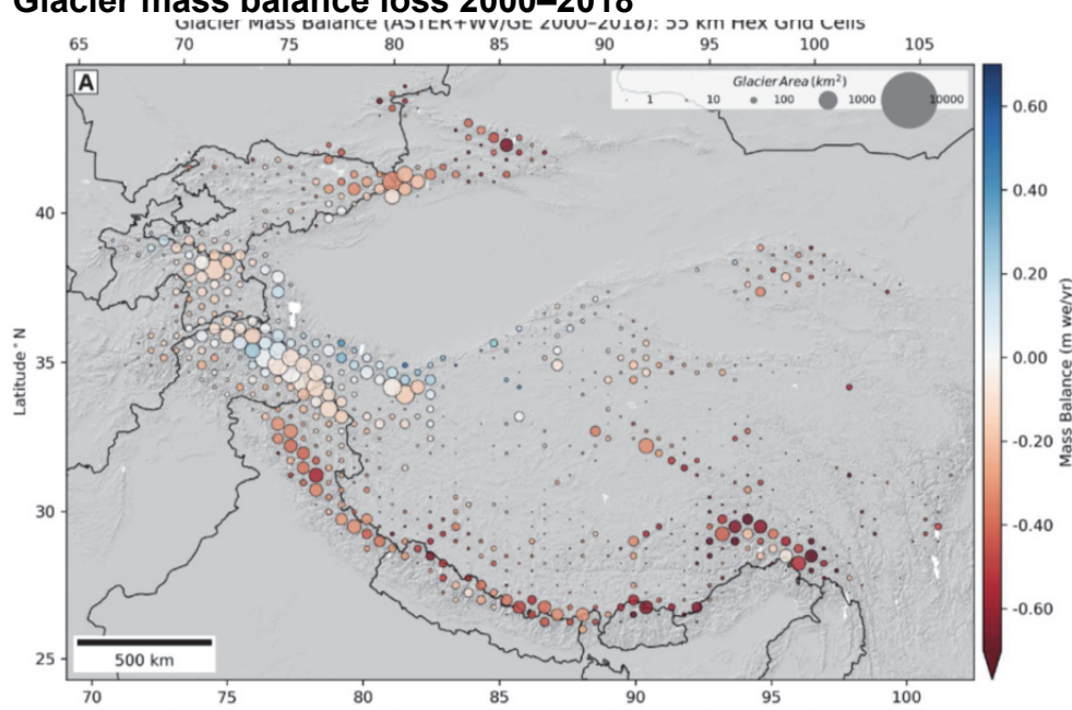
Figure 7 Glacier mass balance loss 2000–2018
