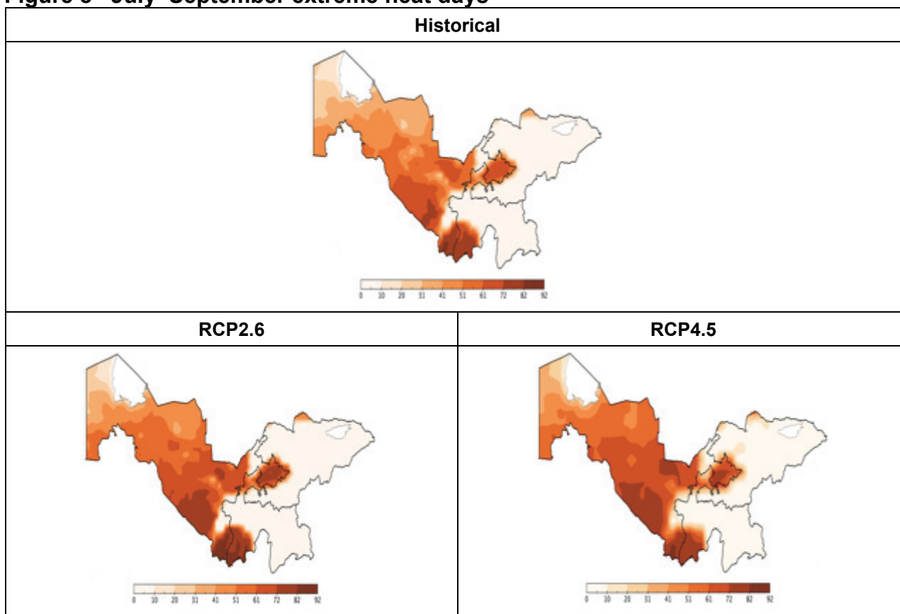
Figure 8 July–September extreme heat days
