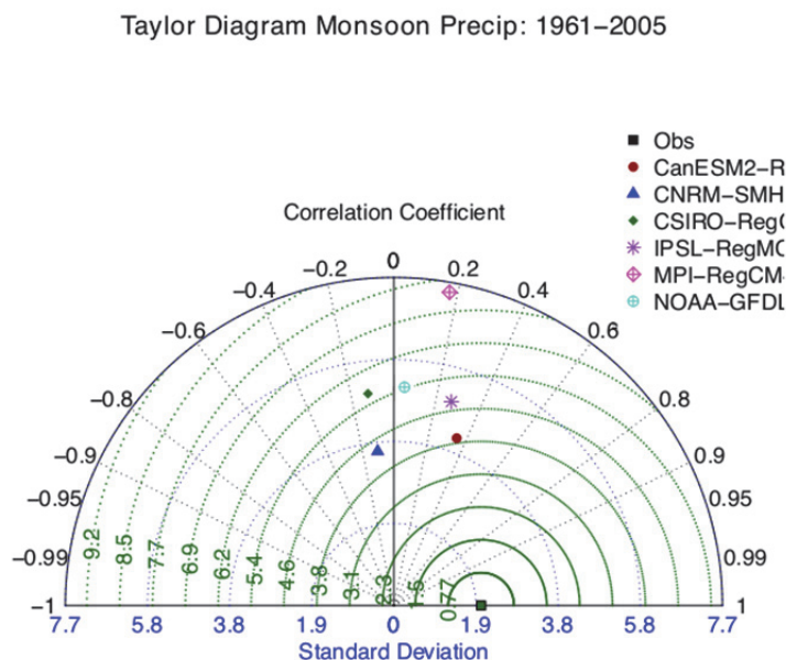
Figure 11 Taylor diagram
