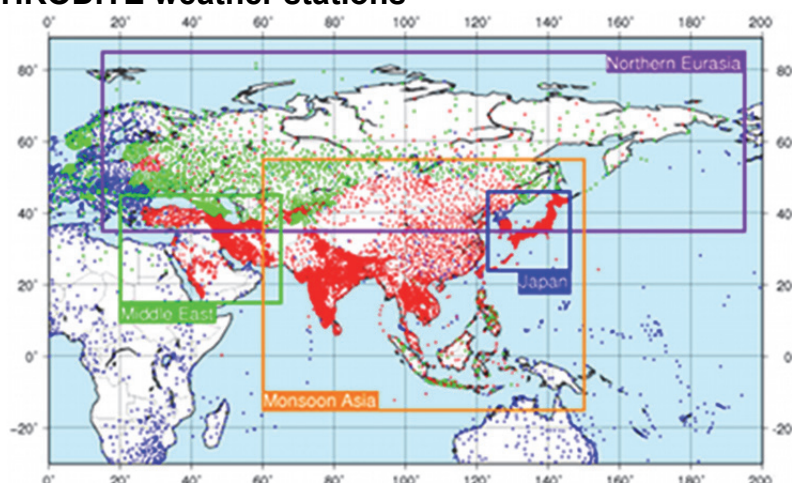
Figure 10 APHRODITE weather stations
