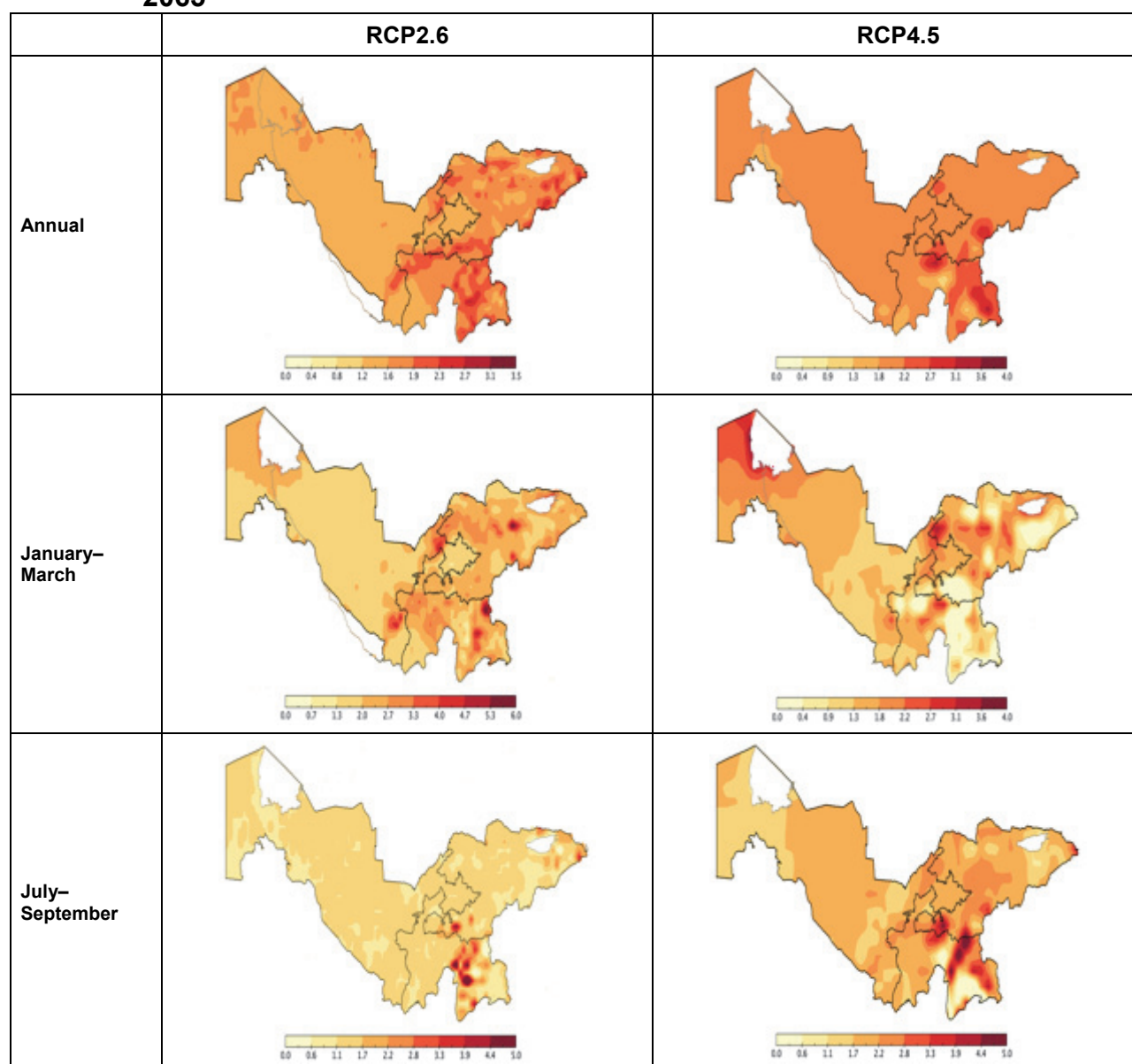
Figure 6 Projected anomalies in annual and seasonal minimum temperatures 2041–2065
