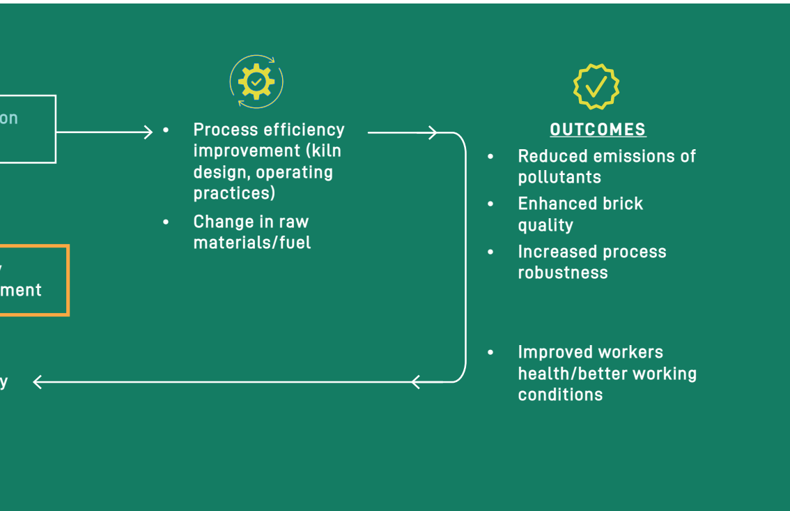
Figure 1.6: GeoAI Overview
